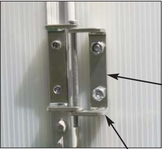
Lower hinge ( Outside greenhouse) Hinge-half on door sits below hinge-half on door casing.
