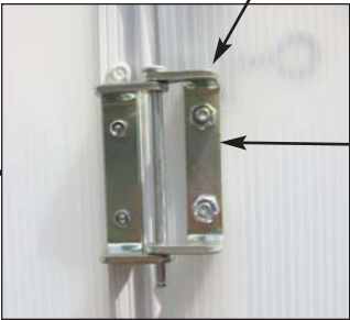
Upper hinge ( Outside greenhouse) Hinge-half on door sits above hinge-half on door casing.
