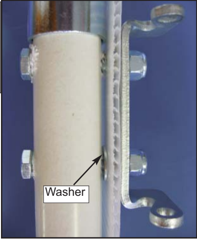
Side view of assembled upper hinge-half on door
