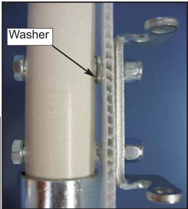
Side view of assembled lower hinge-half on door
