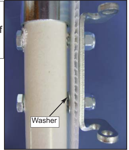
Side view of assembled upper hinge-half on door →
