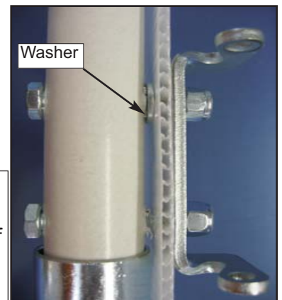
Side view of assembled lower hinge-half on door →
